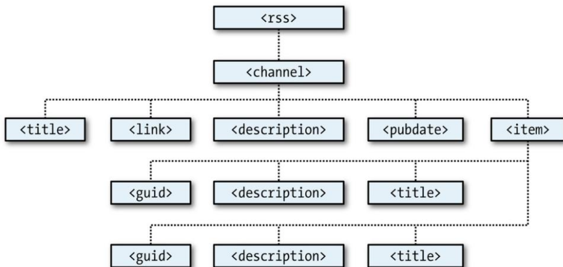
Figure 18-3. The DOM tree of Example 18-8
